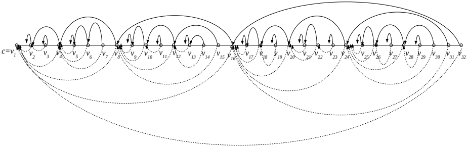
Fig. 3. Secondary structures of the nodes in \mathcal{T}
