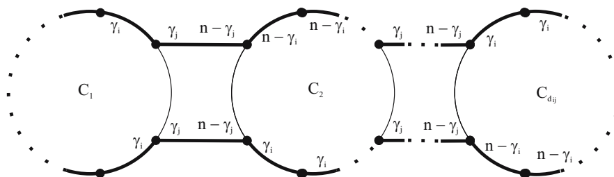
Fig. 3. Larger cycle using the cycles whose edges are labeled with \gamma_i and edges labeled with \gamma_j
