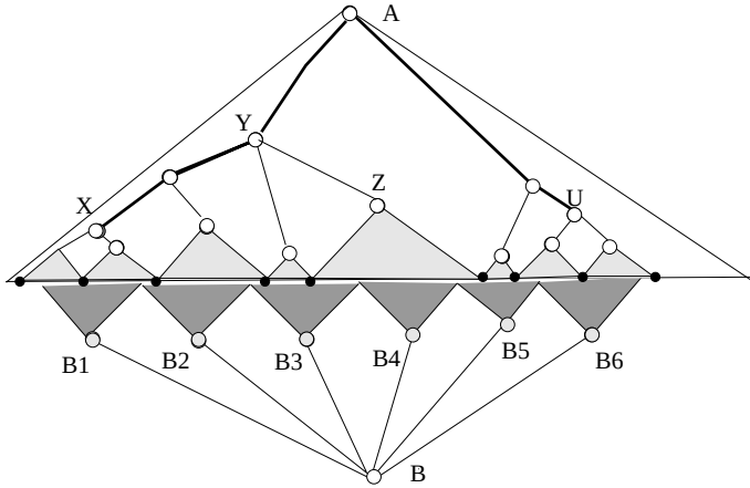
Fig. 2. (A, B1, *) is covered by (X, B1, *, *) , (A, B4, *) is covered by (B, Z, *, *) and (A, B3, *) is covered by (Y, B3, *, *) , the * 's denote corresponding positions in the items. The set \mathcal{S} consists of small darkened circles.
