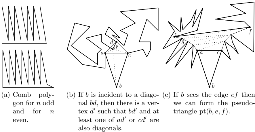
Fig. 7. Lower bound (a). An example 24-gon. (b)-(c).
