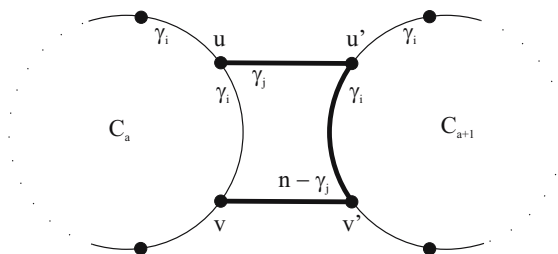
Fig. 2. A path connecting vertices u and v and whose edges are labeled with \gamma_j , \gamma_i , and n - \gamma_j (in this order). Cycles C_a and C_{a+1} belong to the 2-factor whose edges are labeled with \gamma_i .
