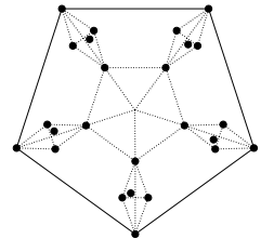
Fig. 5. Lower bound example for k = 5
